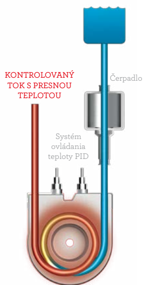
Thermocoil
